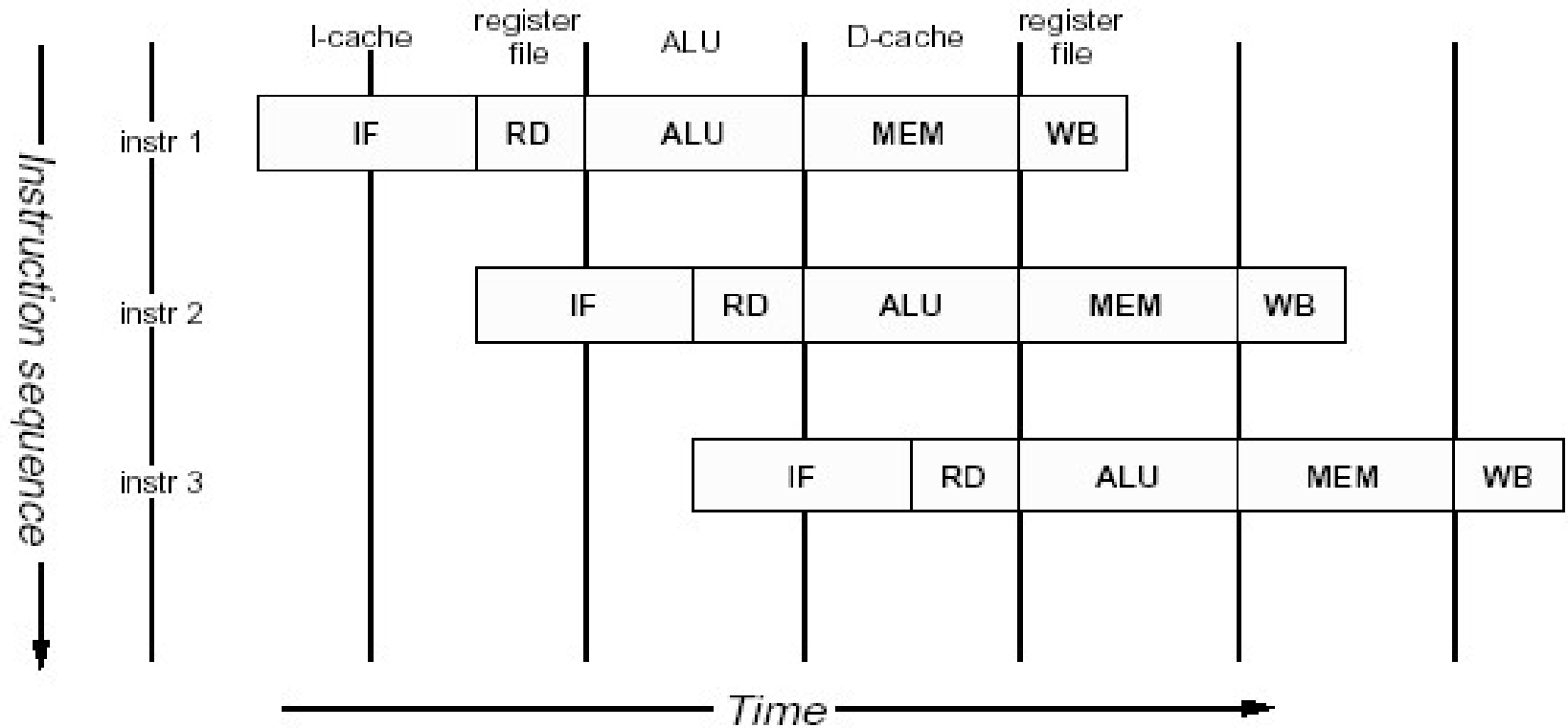
Figure 1.1. MIPS 5-stage pipeline
